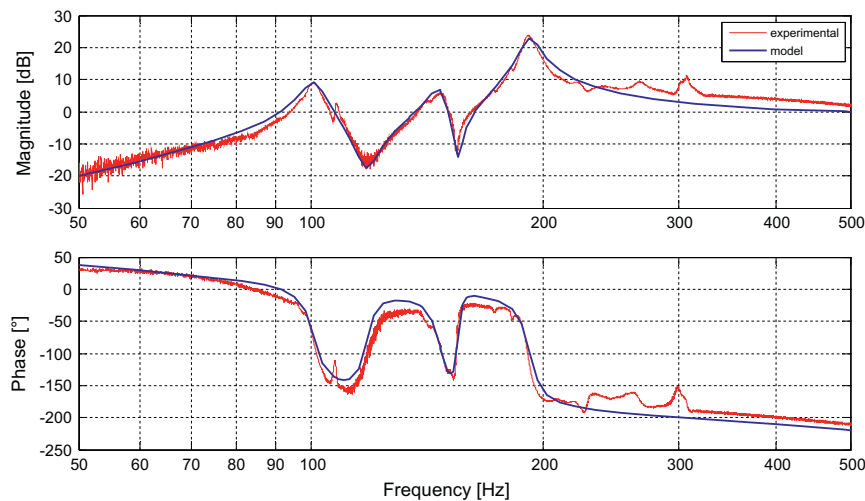
Fig. 7. Comparison between the experimental and the estimated Bode plots of G_{av}(s) .
